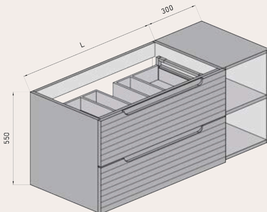
Front view FURNITURE PLUS SHELF MODULE
